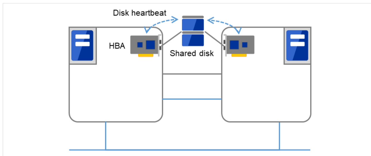
Fig. 3.4: Disk heartbeat
