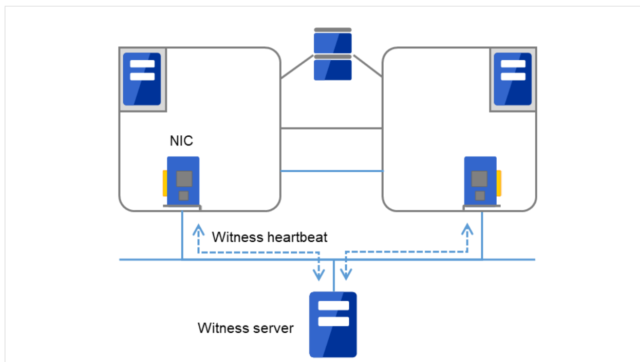
Fig. 3.5: Witness heartbeat
